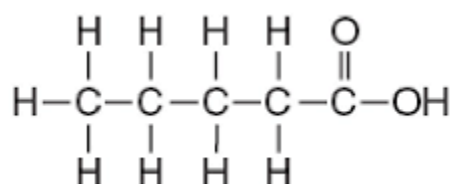
Pentanoic acid
